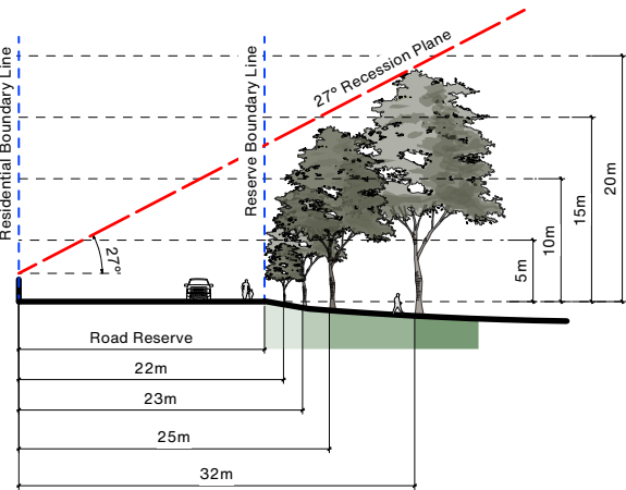
Cross Section G-G
