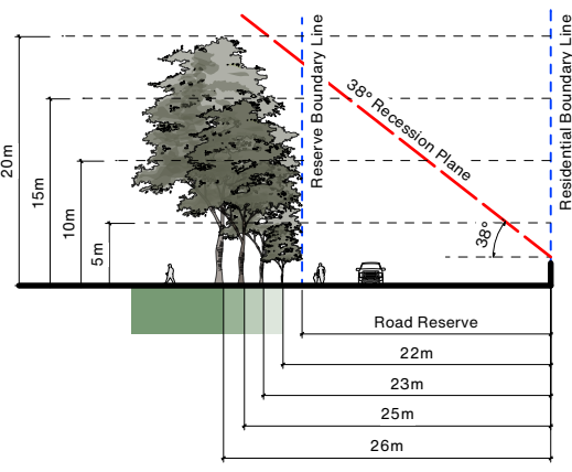
Cross Section K-K
