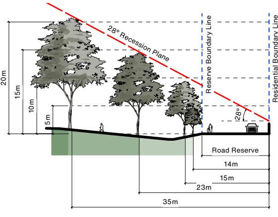
Cross Section J-J
