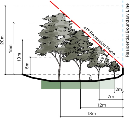
Cross Section D-D
