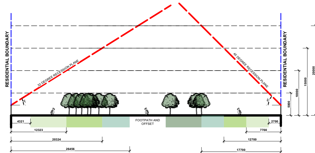
G BOUNDARY SECTION G-G Scale: 1:500
