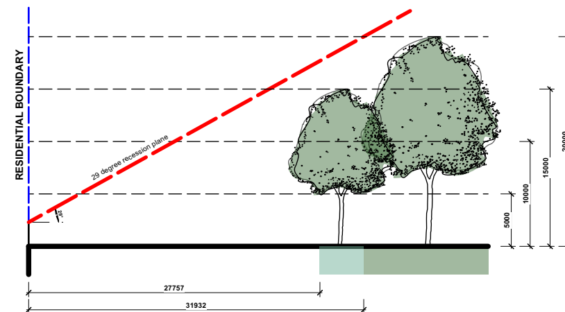
H BOUNDARY SECTION H-H Scale: 1:500
