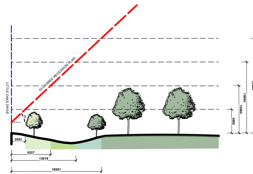
M BOUNDARY SECTION M-M Scale: 1:500
