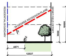
K BOUNDARY SECTION K-K Scale: 1:500
