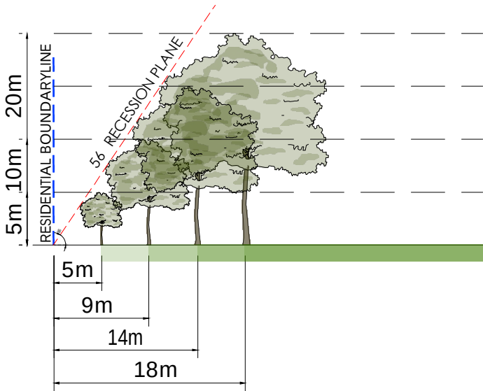
CROSS SECTION JJ
