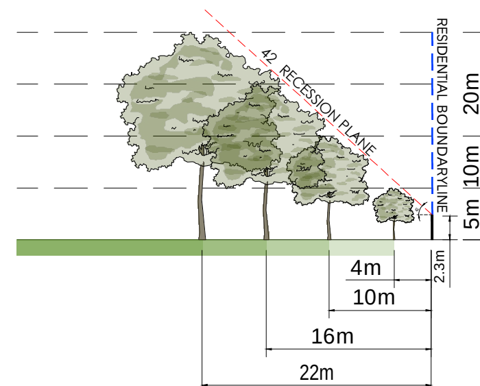
CROSS SECTION CC
