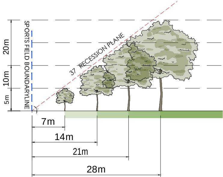
CROSS SECTION II
