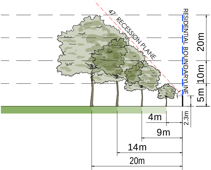
CROSS SECTION GG
