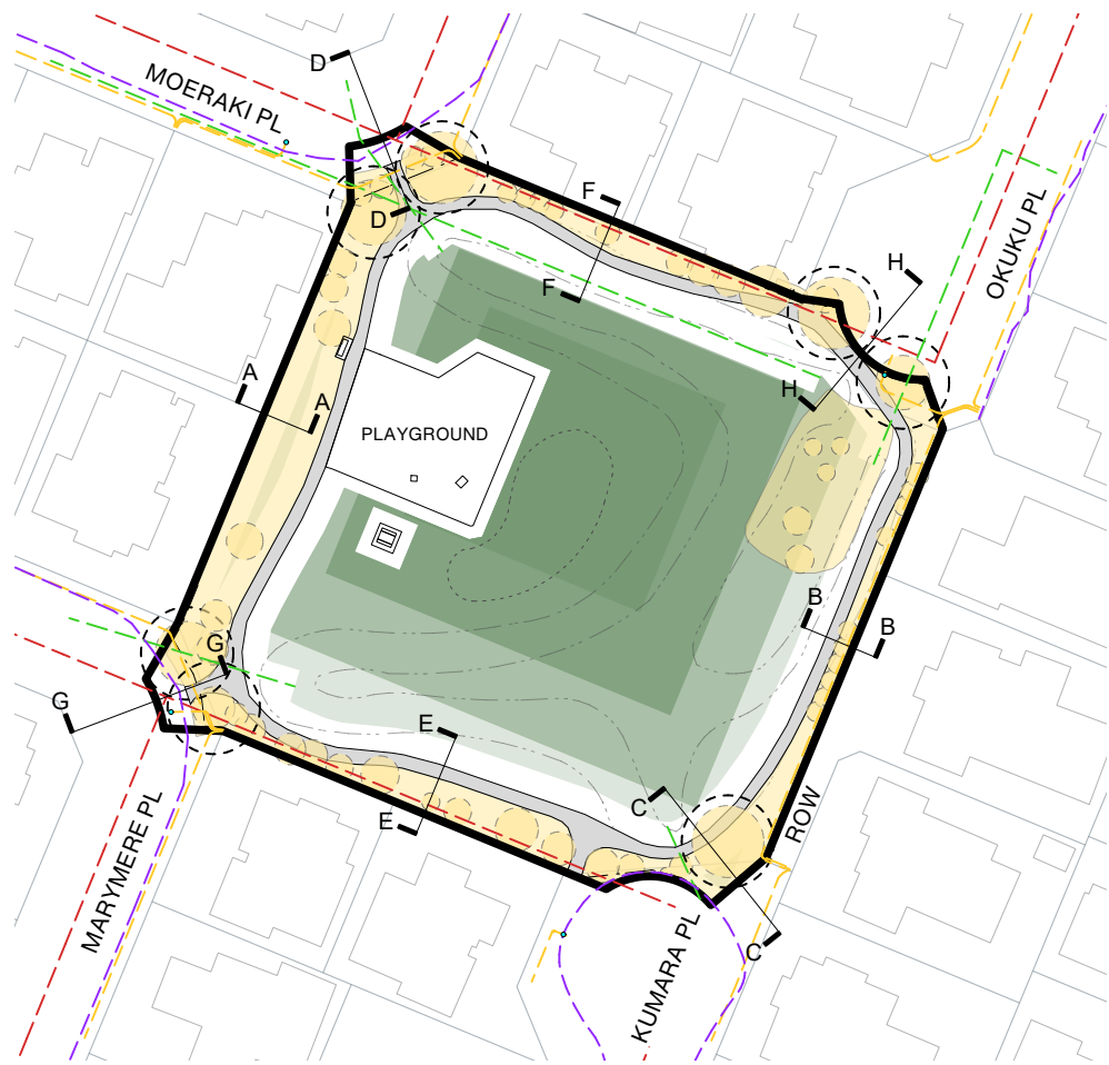
Location Plan @ 1:1500
