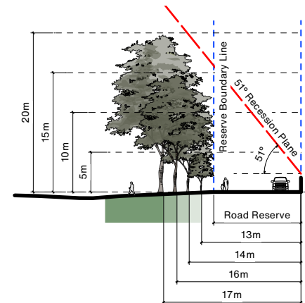
Cross Section D-D
