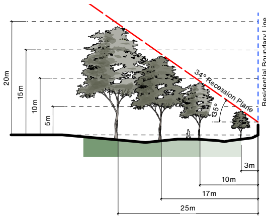
Cross Section B-B
