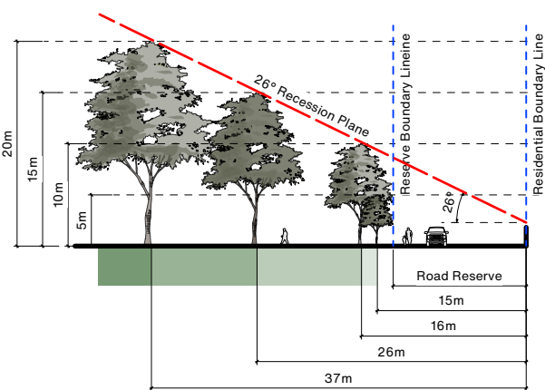
Cross Section D-D
