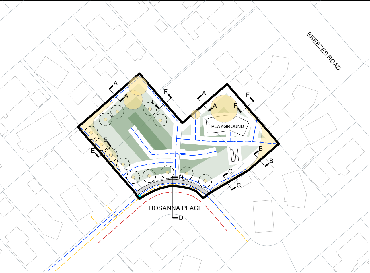
Location Plan @ 1:1000
