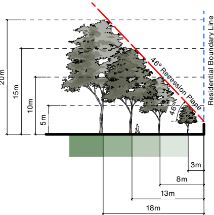
Cross Section F-F
