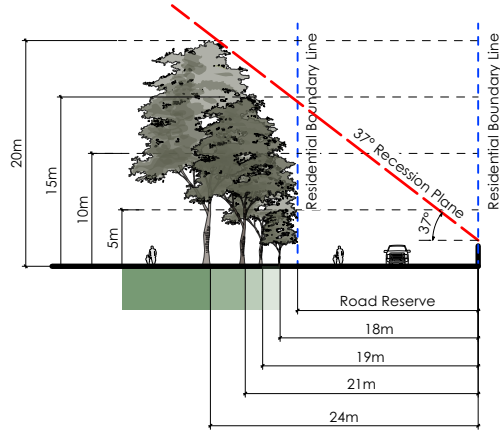
Cross Section E-E
