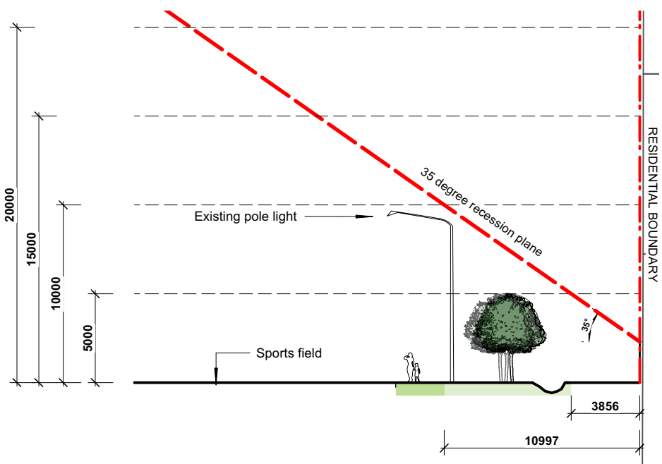
2 BOUNDARY SECTION 2 Scale: 1:300
