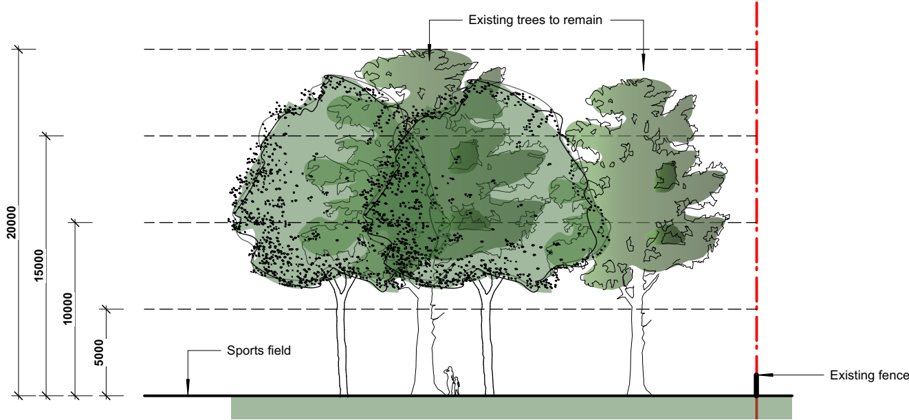
3 BOUNDARY SECTION 3 Scale: 1:300
