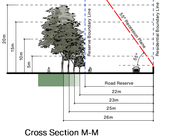
Cross Section P-P
