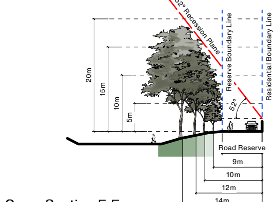
Cross Section K-K
