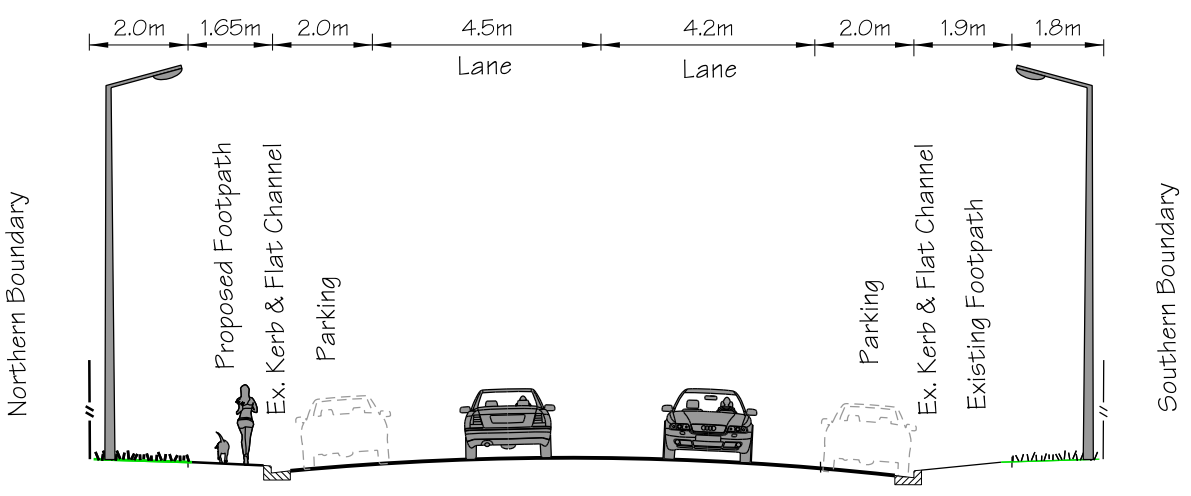
Section A
